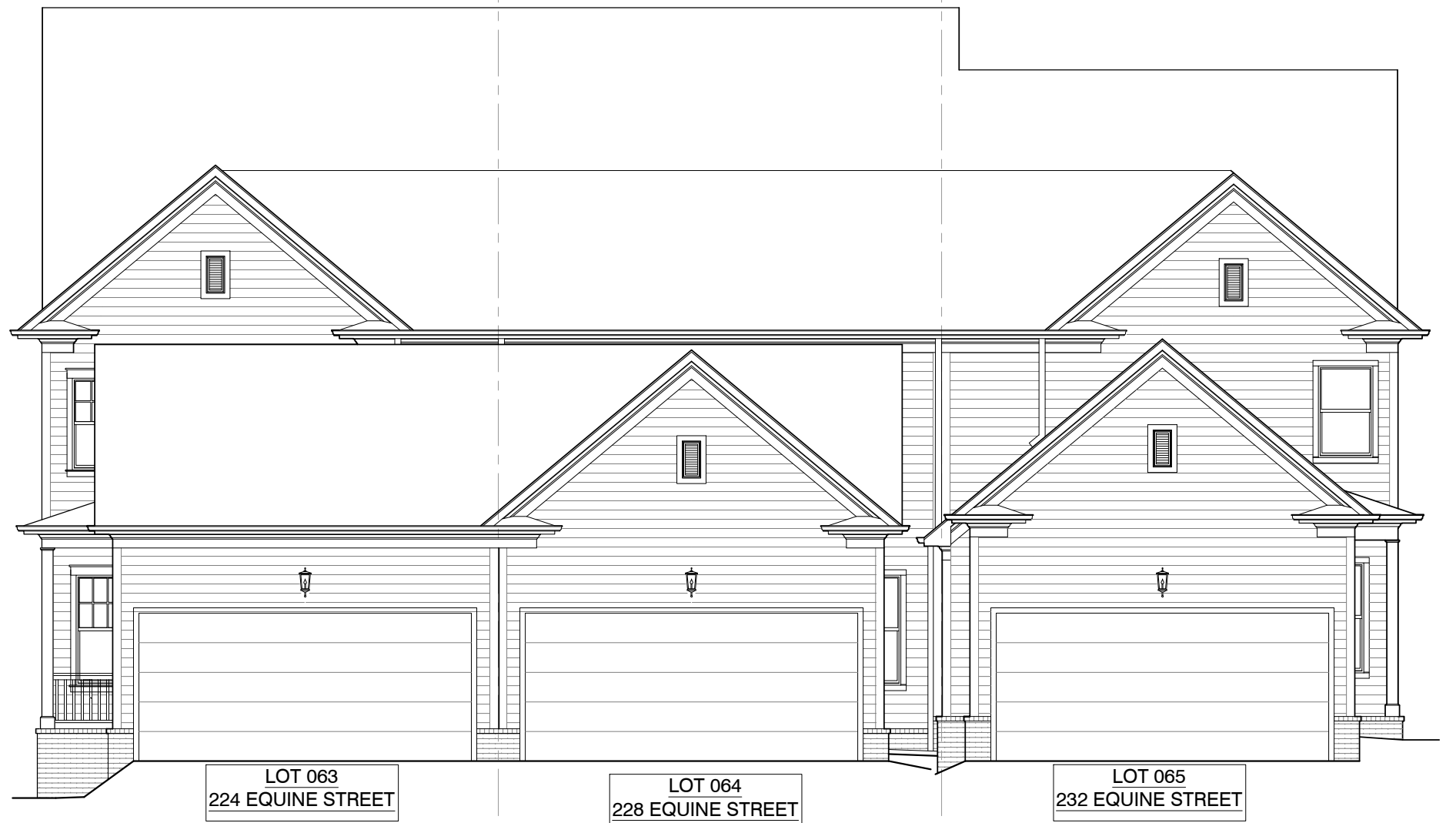
2 REAR ELEVATION 1/8" = 1'-0"
